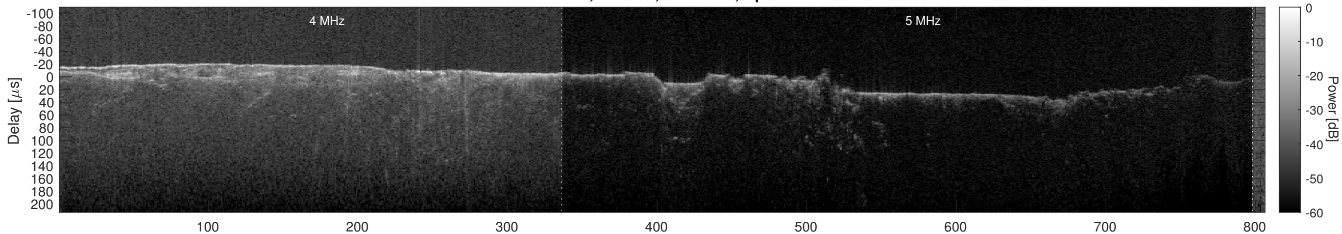
Orbit 14804, Cluttergram
