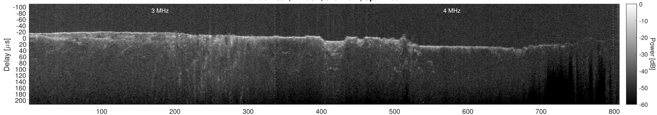
Orbit 14804, Cluttergram
