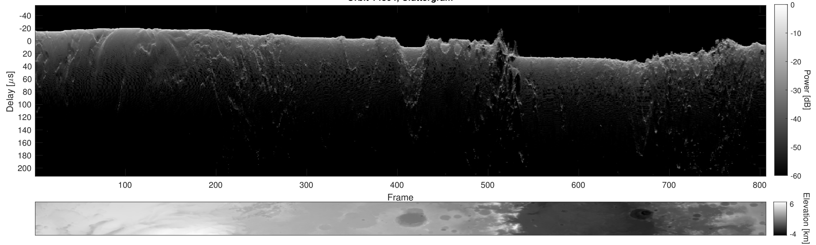
Orbit 14804, Cluttergram
