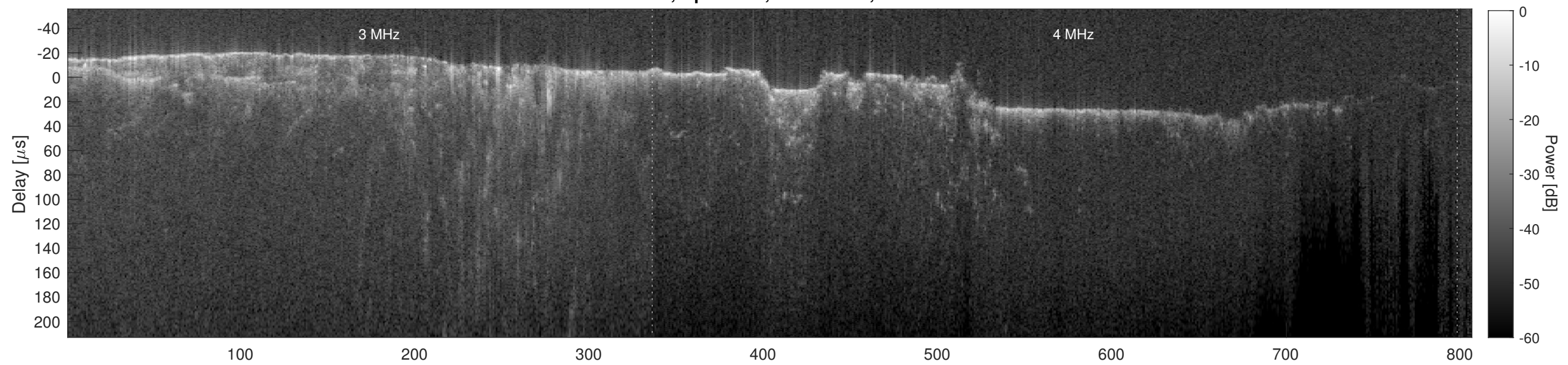
Orbit 14804, Cluttergram
