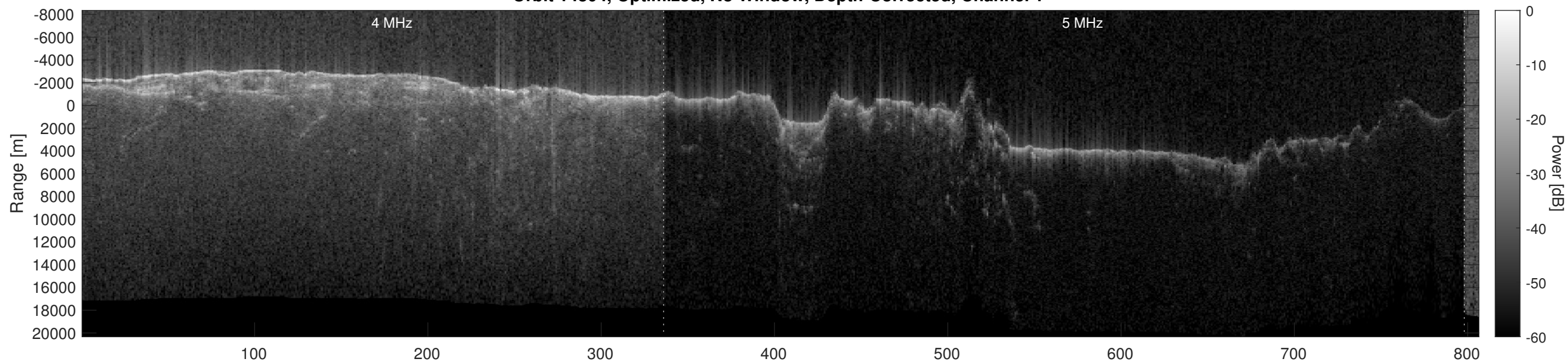
Orbit 14804, Optimized, No Window, Depth-Corrected, Channel 2
