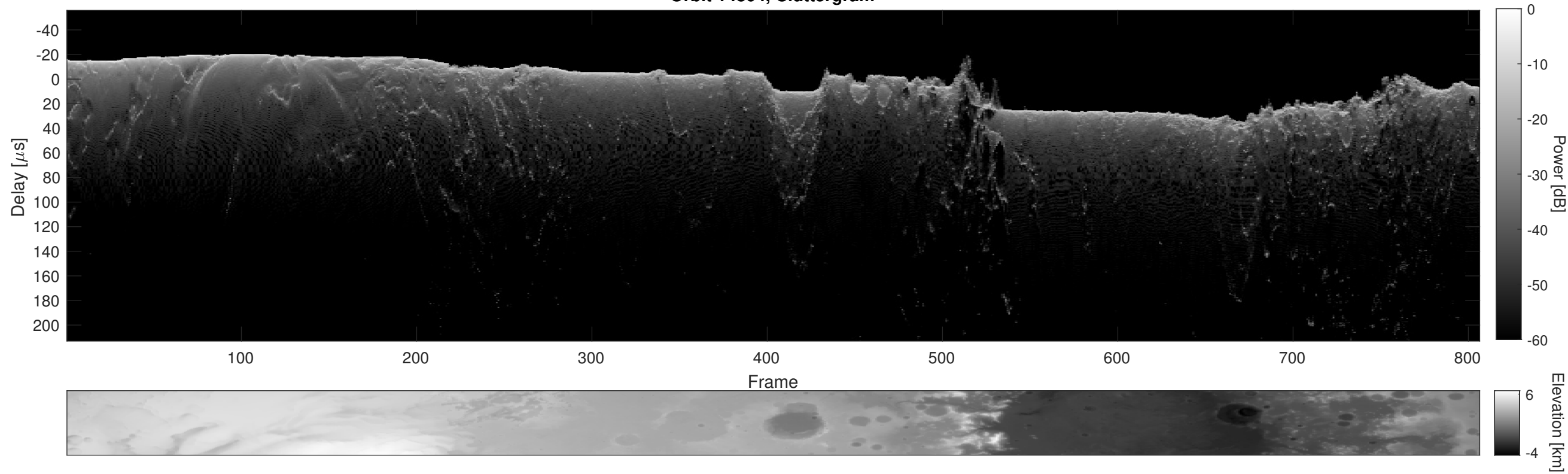
Orbit 14804, Cluttergram
