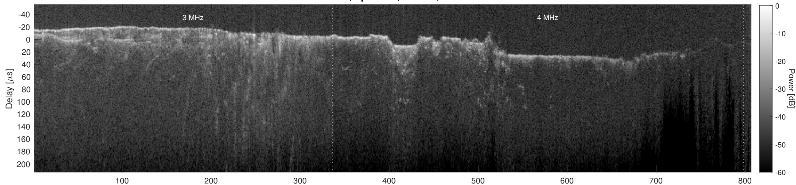
Orbit 14804, Cluttergram
