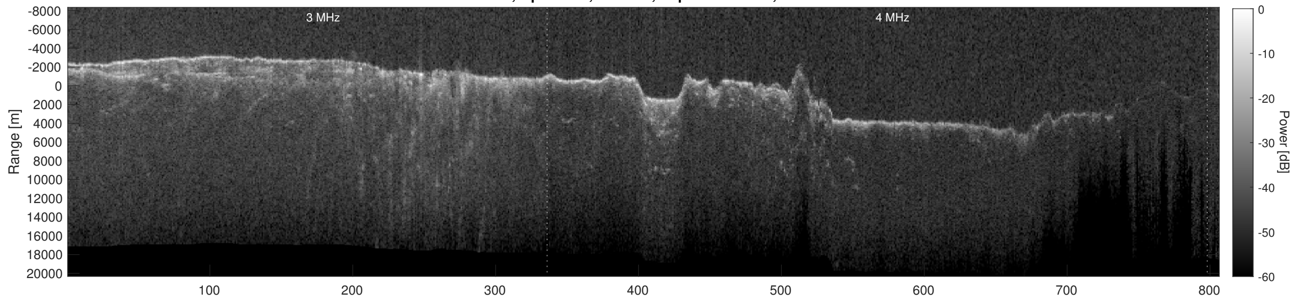
Orbit 14804, Depth-Corrected Cluttergram
