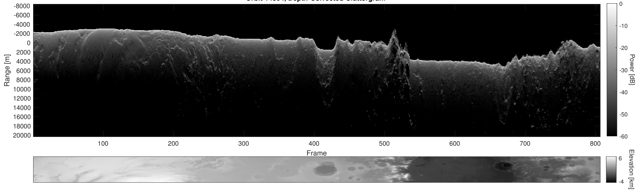
Orbit 14804, Depth-Corrected Cluttergram
