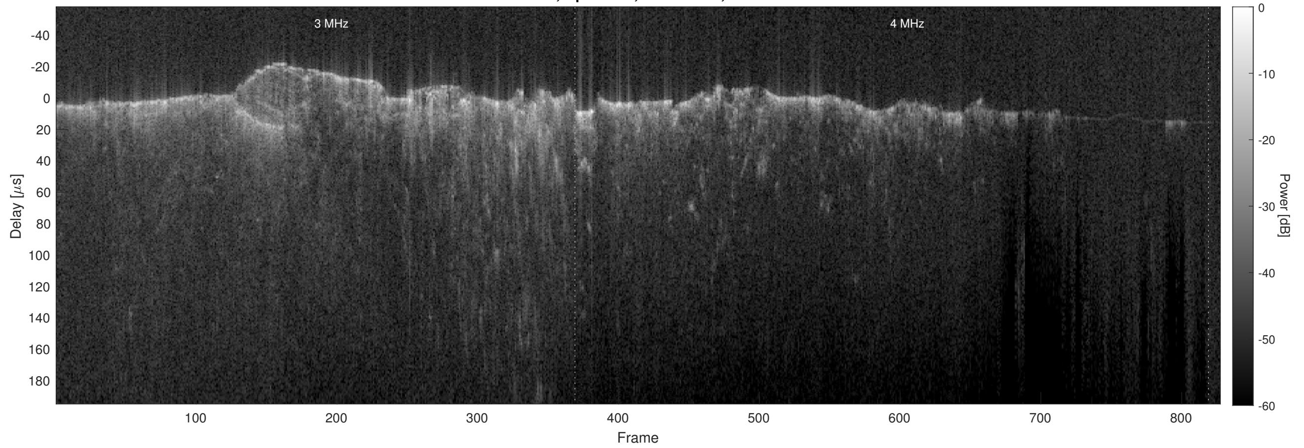
Orbit 14820, Optimized, No Window, Channel 2
