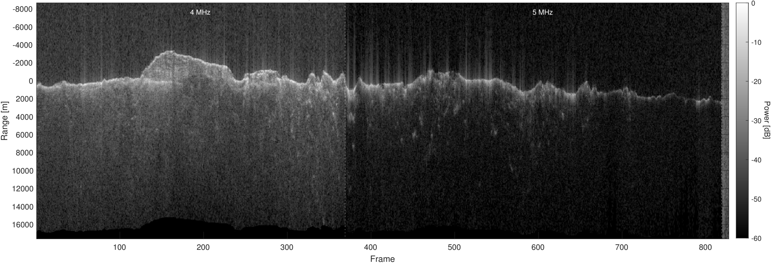
Orbit 14820, Optimized, No Window, Depth-Corrected, Channel 2
