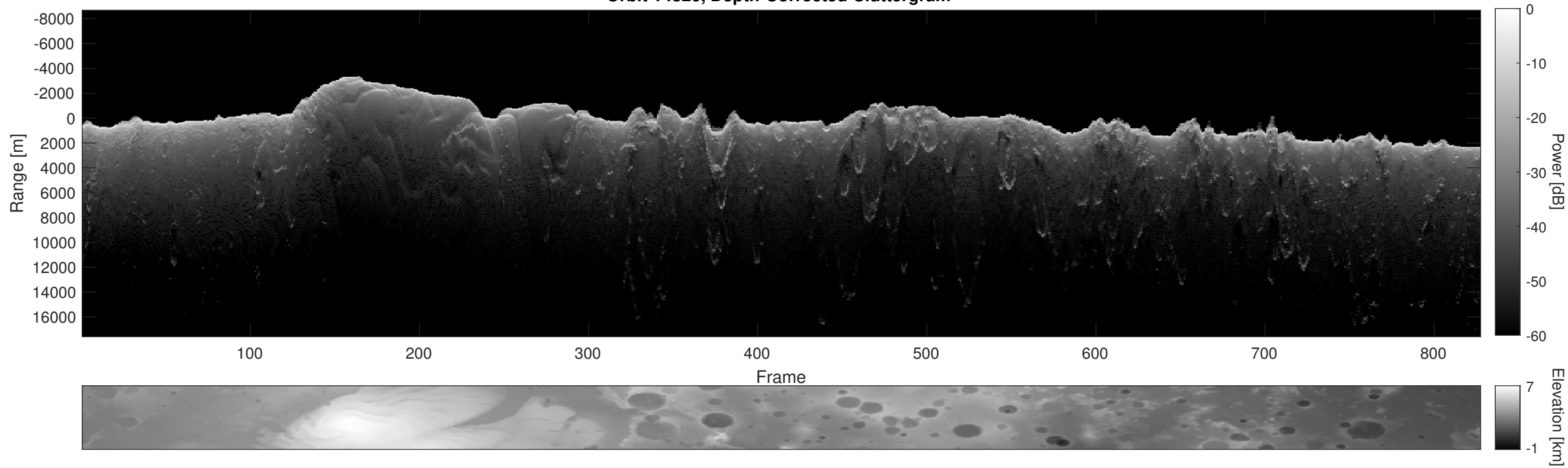
Orbit 14820, Depth-Corrected Cluttergram
