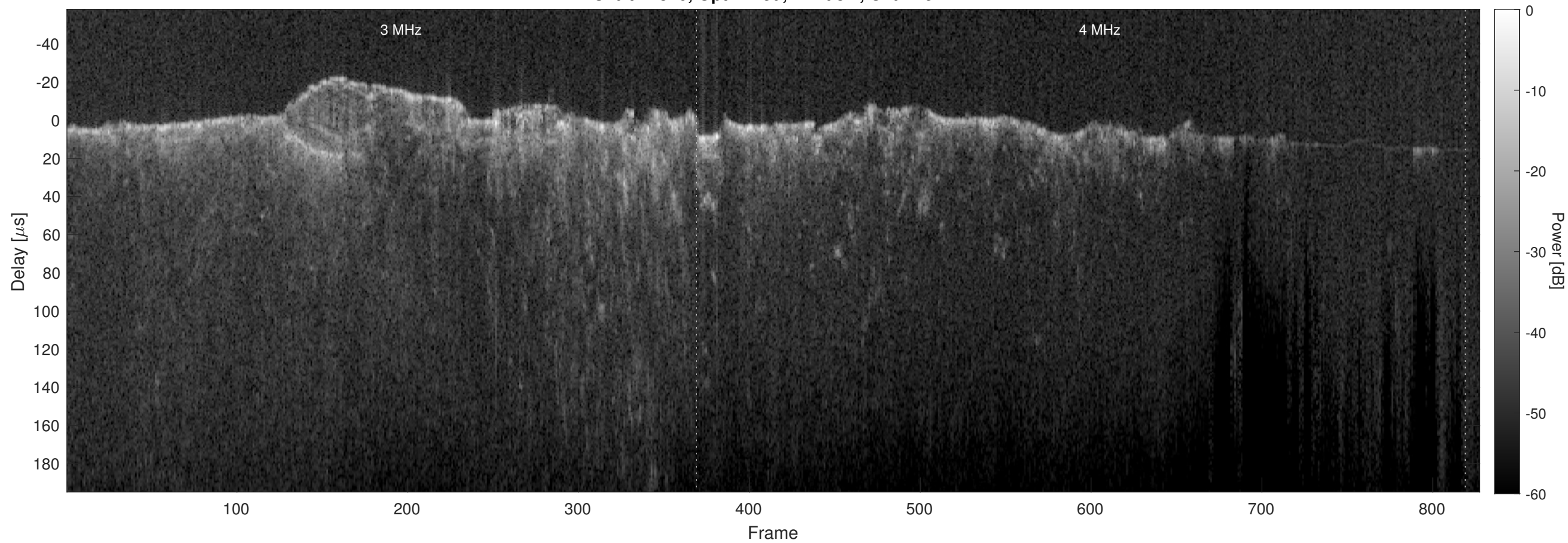
Orbit 14820, Optimized, Window, Channel 2
