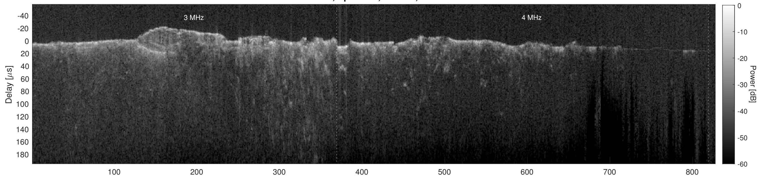
Orbit 14820, Cluttergram
