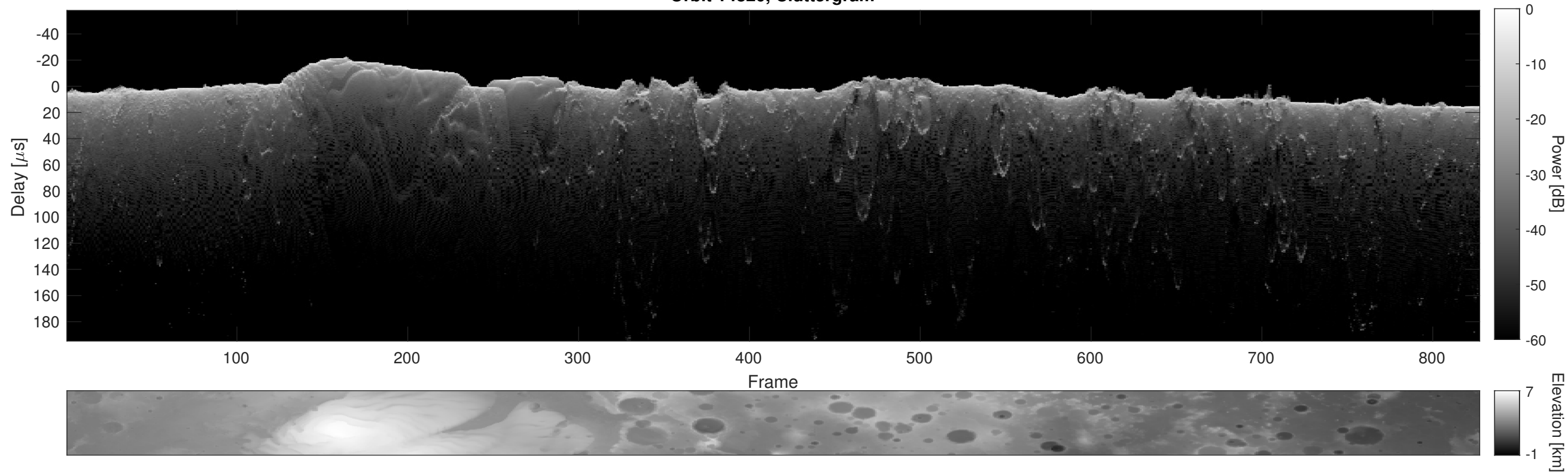
Orbit 14820, Cluttergram
