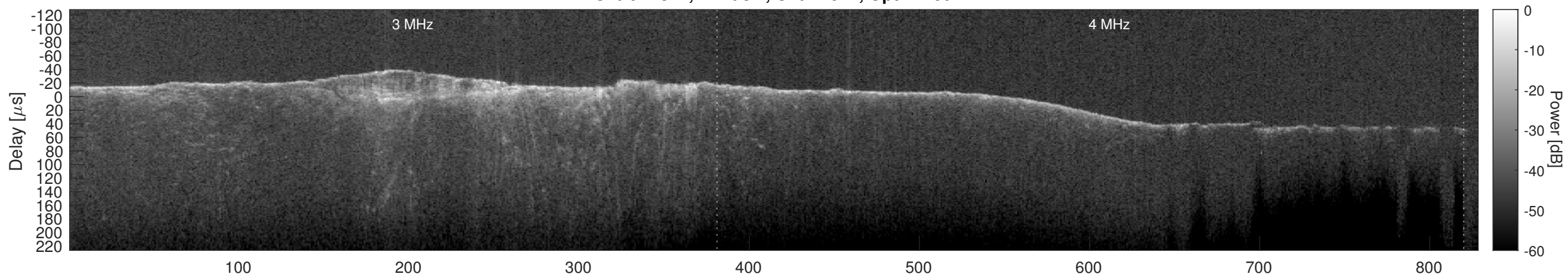
Orbit 14824, Cluttergram
