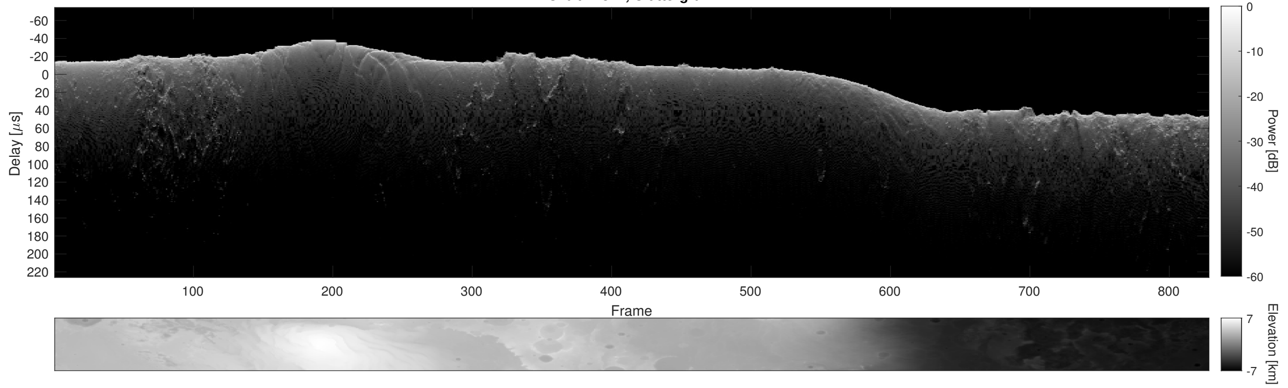
Orbit 14824, Cluttergram
