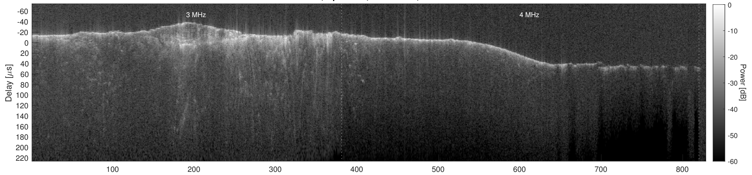
Orbit 14824, Cluttergram
