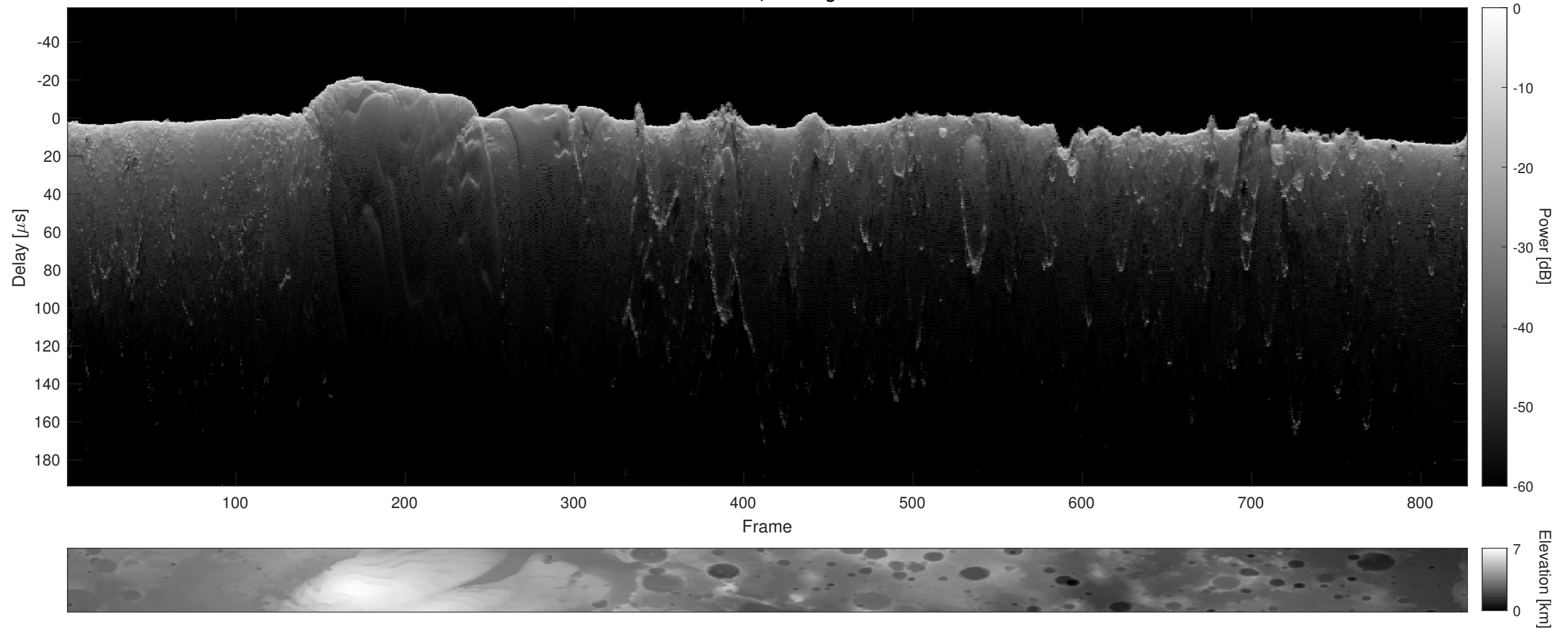
Orbit 14827, Cluttergram
