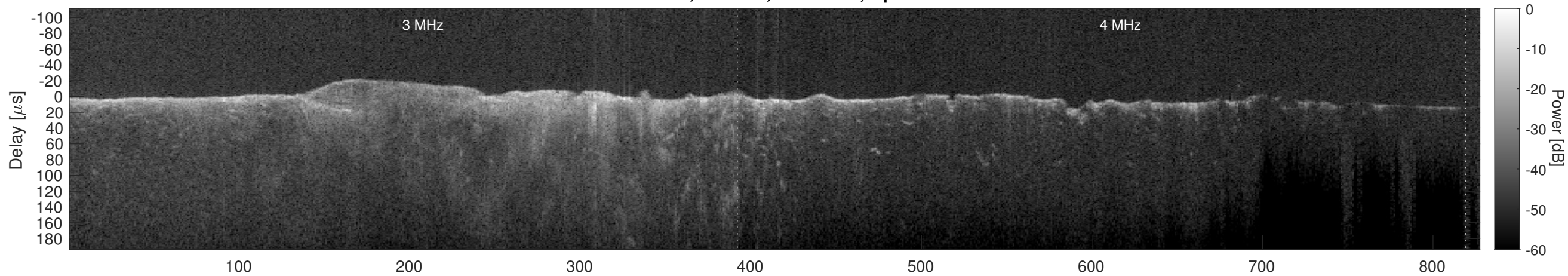
Orbit 14827, Cluttergram
