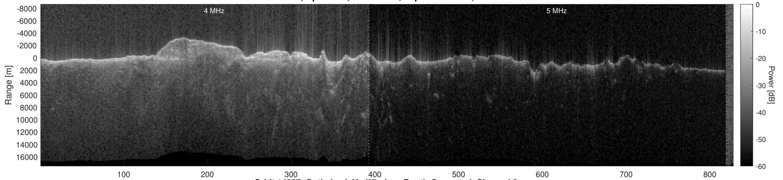
Orbit 14827, Optimized, No Window, Depth-Corrected, Channel 2
