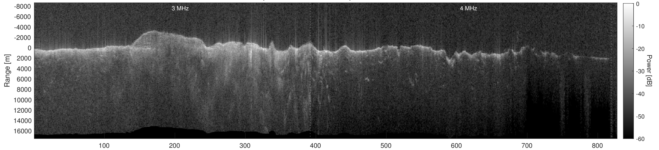
Orbit 14827, Depth-Corrected Cluttergram
