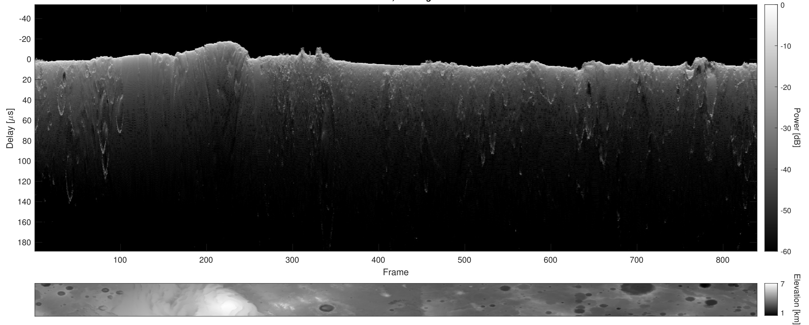
Orbit 14828, Cluttergram
