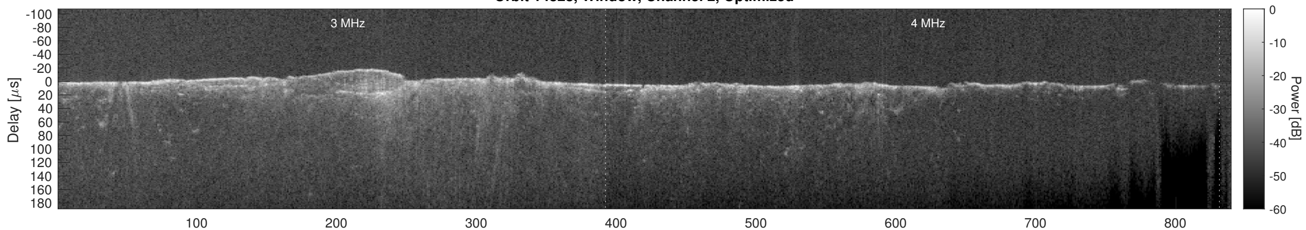
Orbit 14828, Cluttergram
