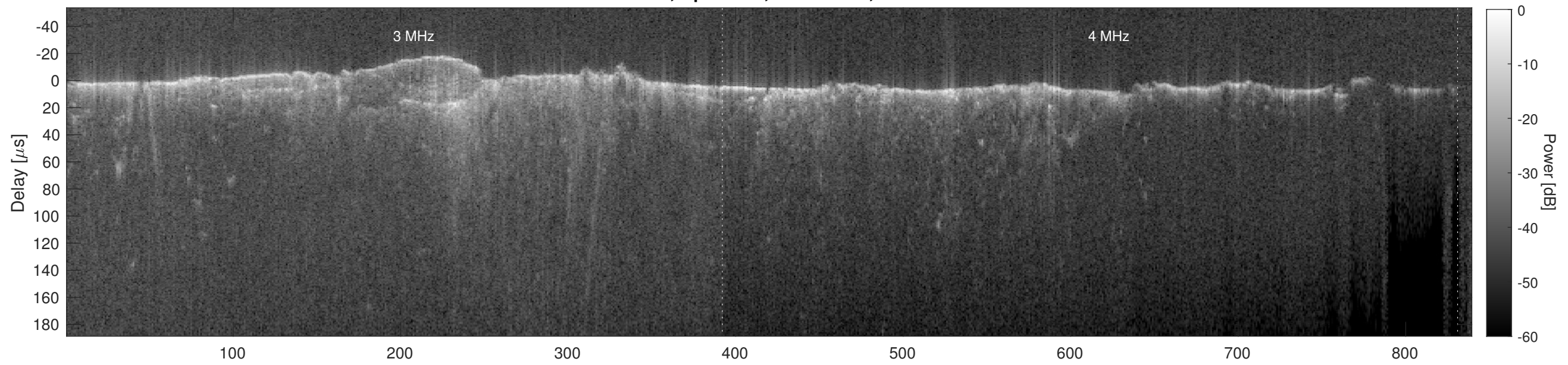
Orbit 14828, Cluttergram
