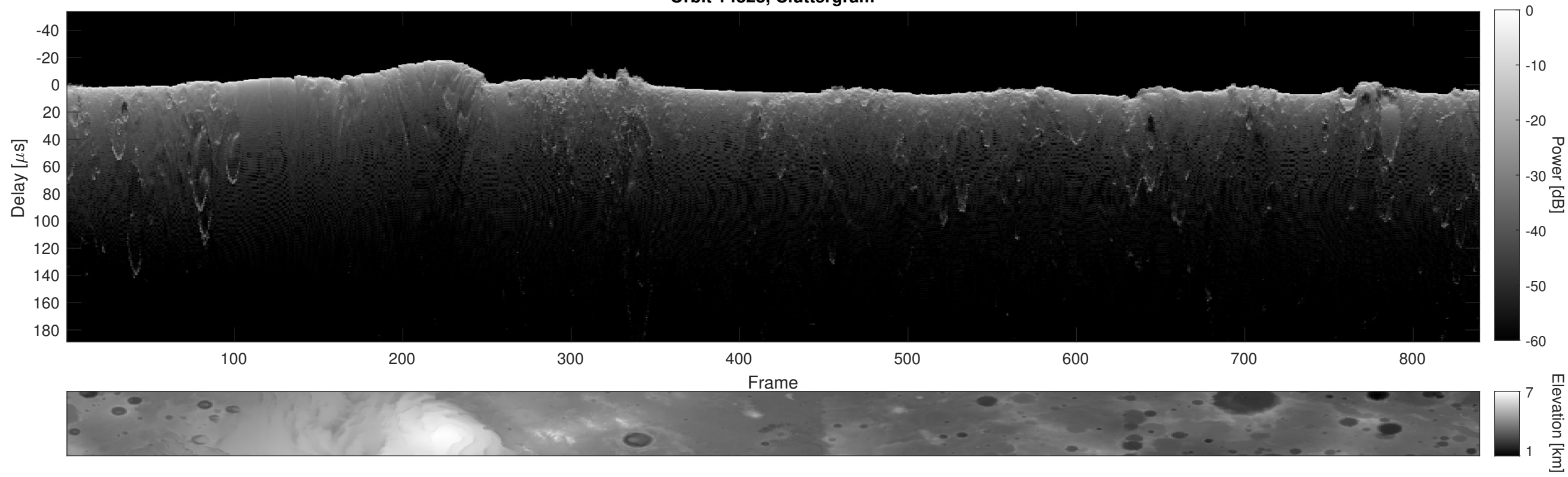
Orbit 14828, Cluttergram
