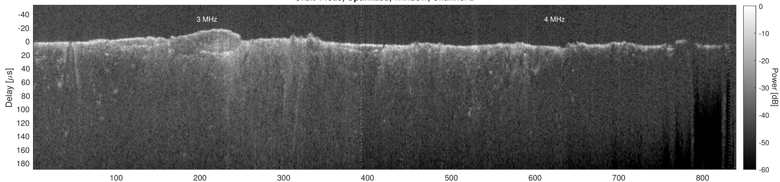
Orbit 14828, Cluttergram
