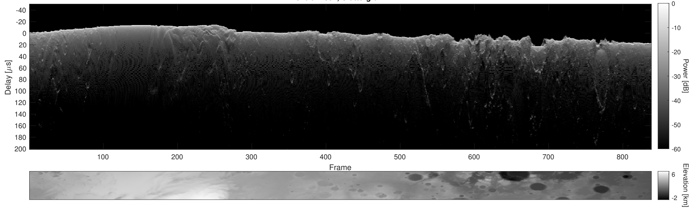
Orbit 14832, Cluttergram
