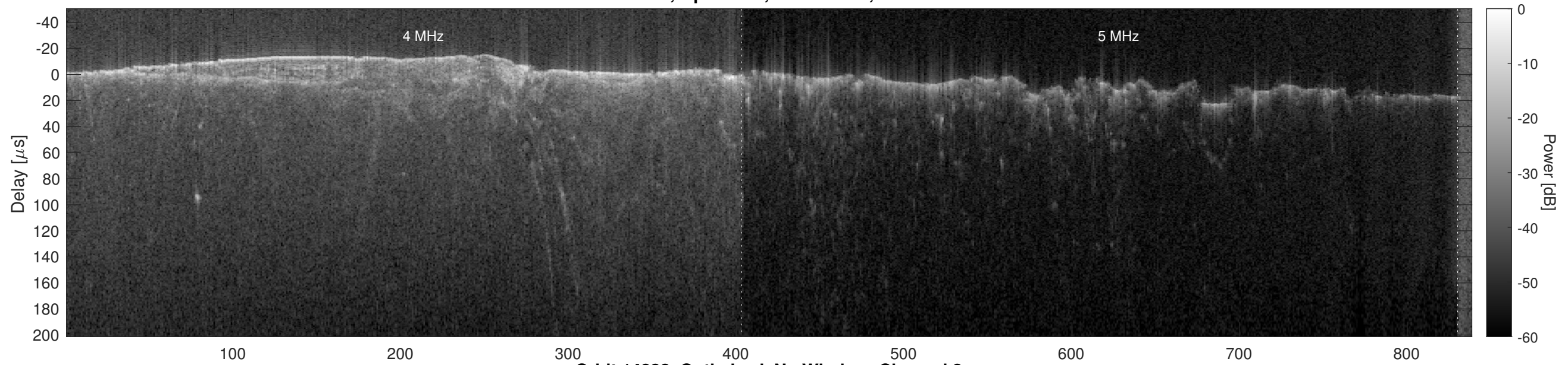
Orbit 14832, Optimized, No Window, Channel 2
