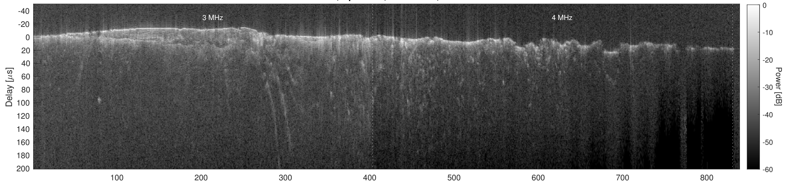
Orbit 14832, Cluttergram
