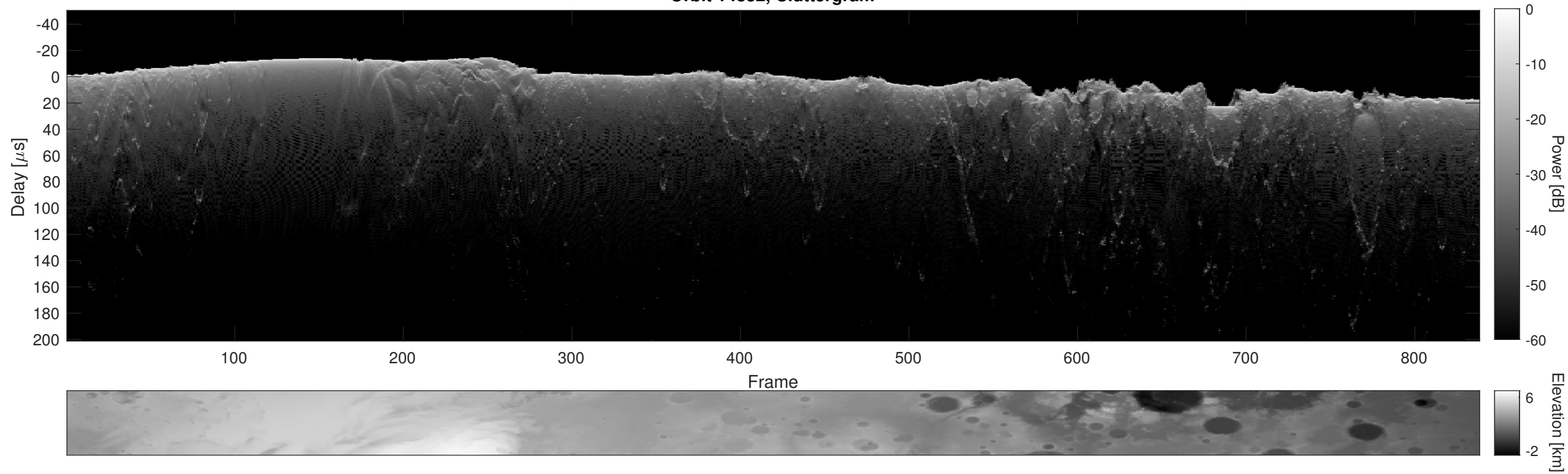
Orbit 14832, Cluttergram
