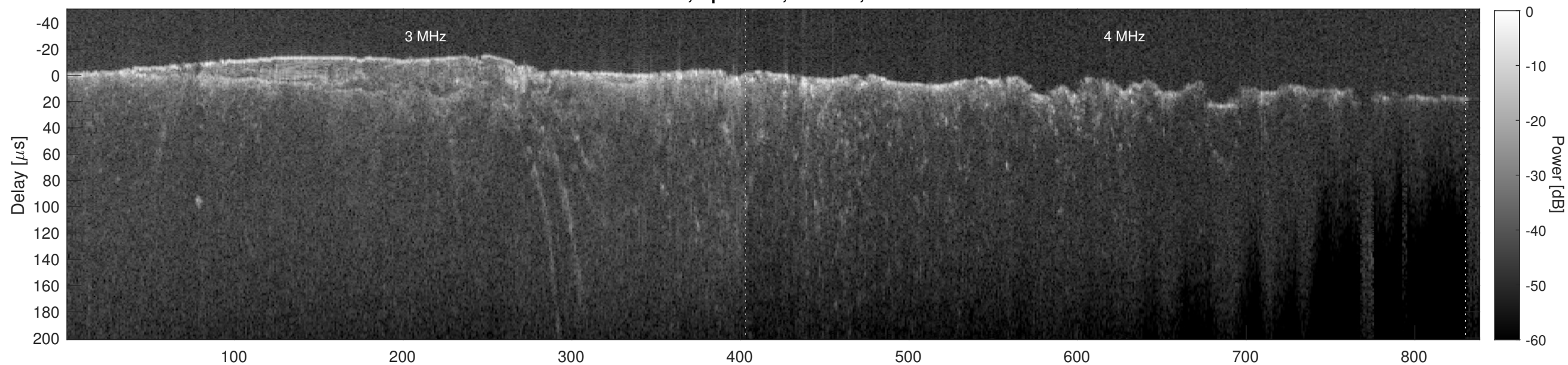
Orbit 14832, Cluttergram
