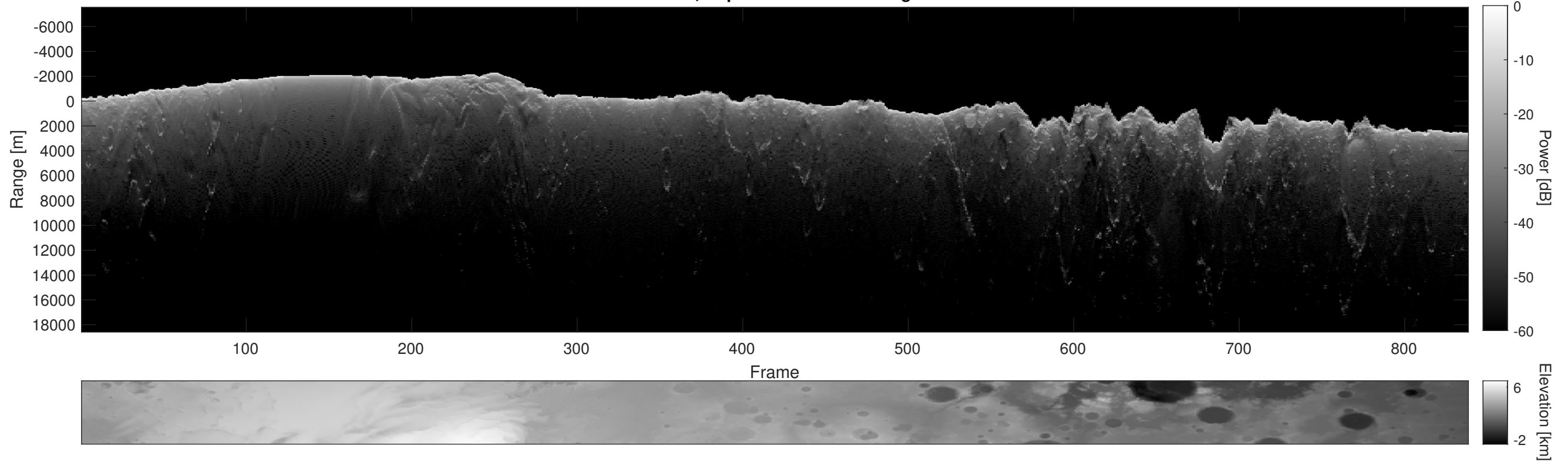
Orbit 14832, Depth-Corrected Cluttergram
