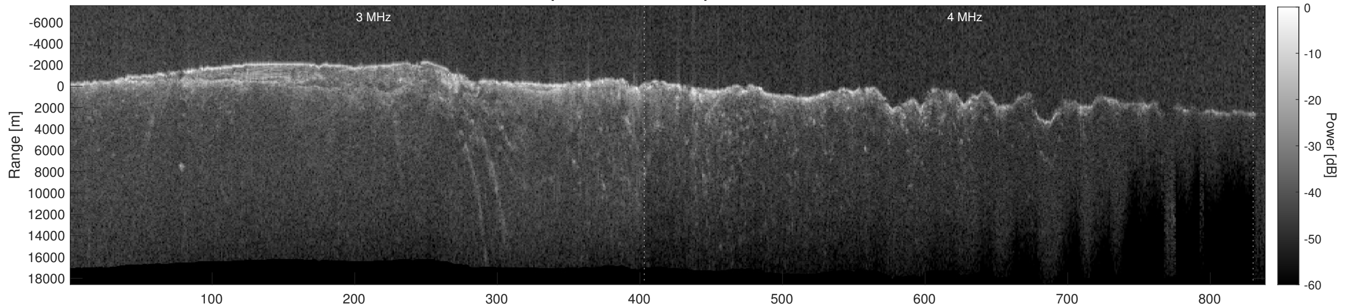
Orbit 14832, Depth-Corrected Cluttergram
