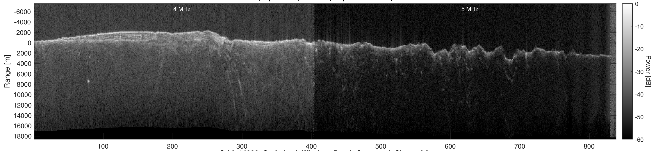
Orbit 14832, Optimized, Window, Depth-Corrected, Channel 2
