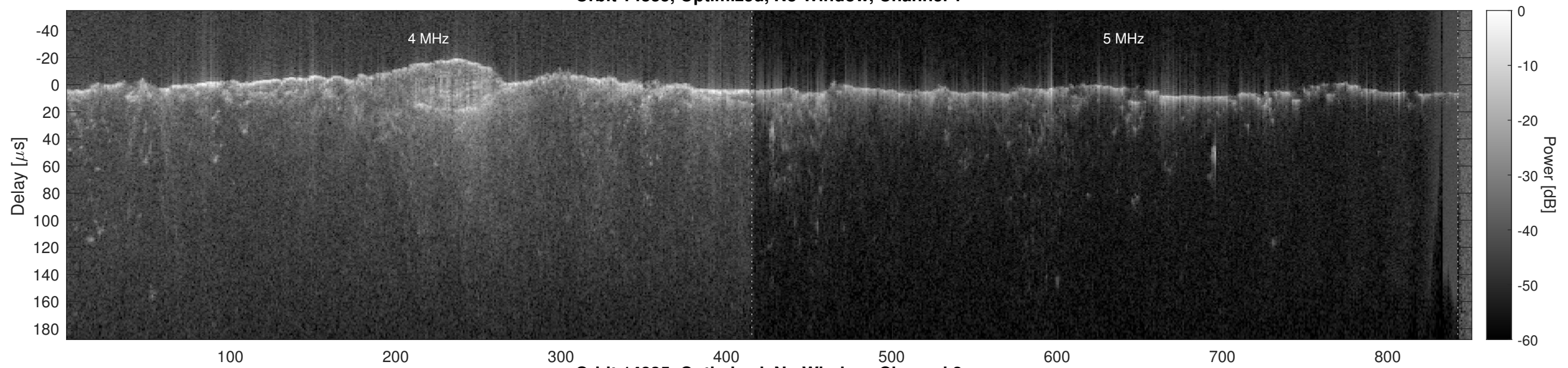
Orbit 14835, Optimized, No Window, Channel 2
