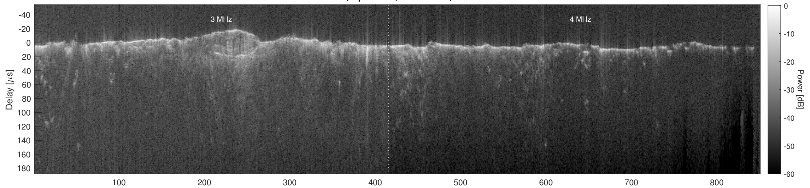
Orbit 14835, Cluttergram
