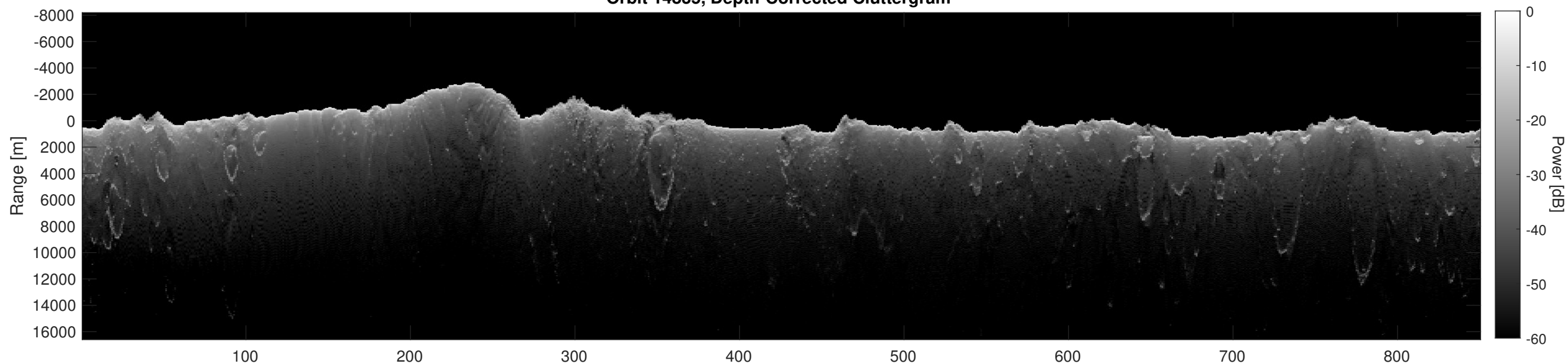
Orbit 14835, Depth-Corrected Cluttergram
