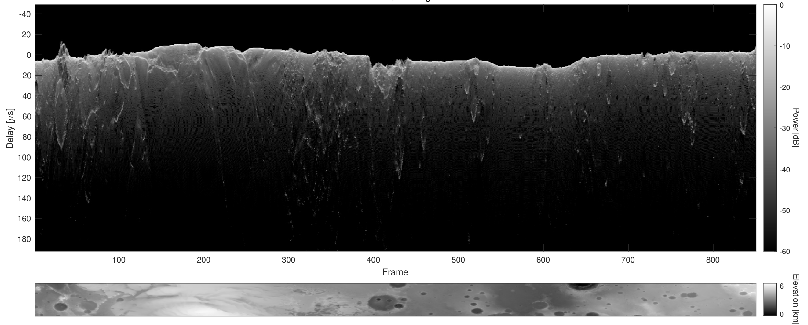
Orbit 14836, Cluttergram
