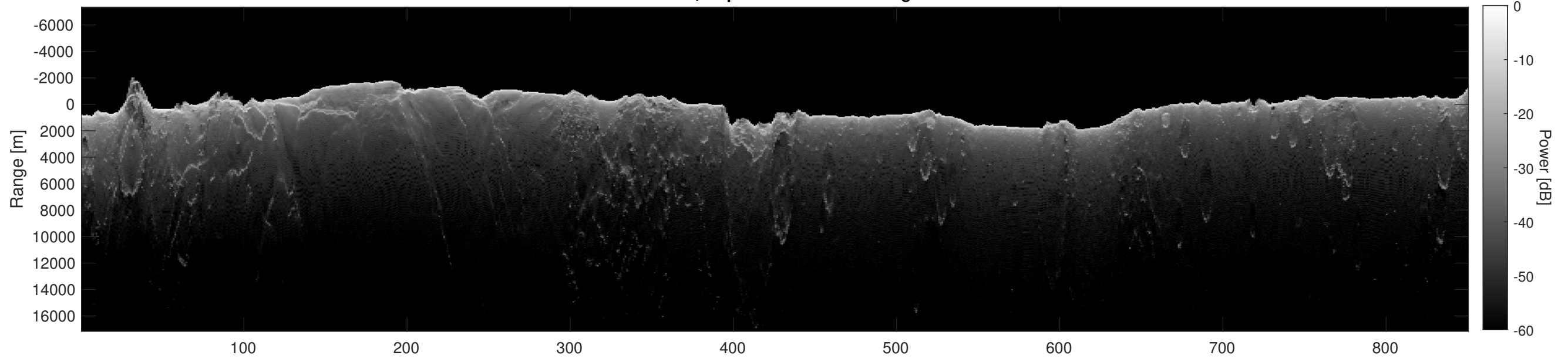
Orbit 14836, Depth-Corrected Cluttergram
