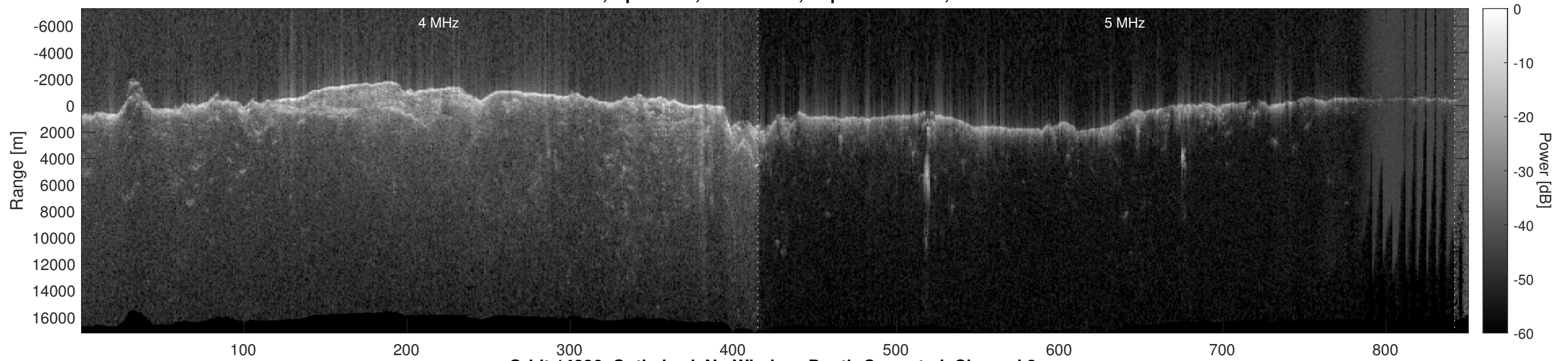
Orbit 14836, Optimized, No Window, Depth-Corrected, Channel 2
