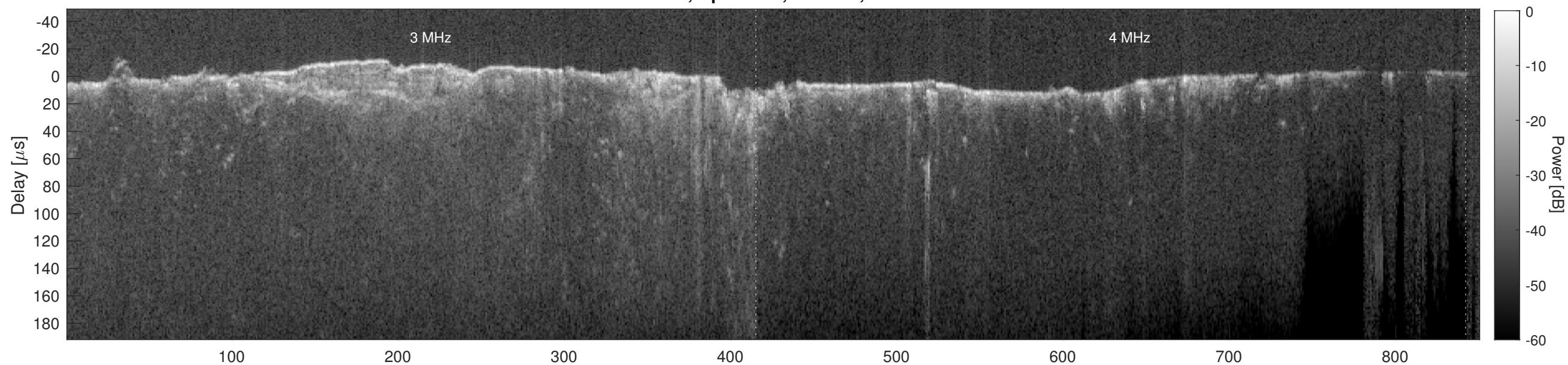
Orbit 14836, Cluttergram
