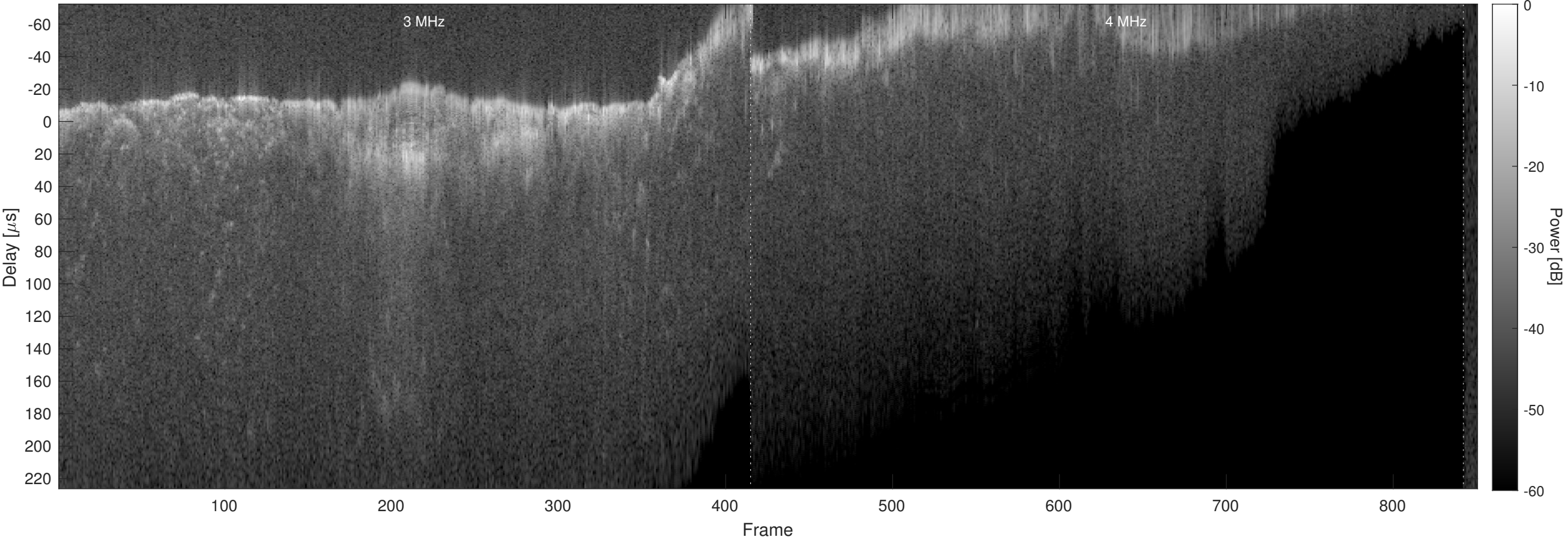
Orbit 14838, Chapman, No Window, Channel 2
