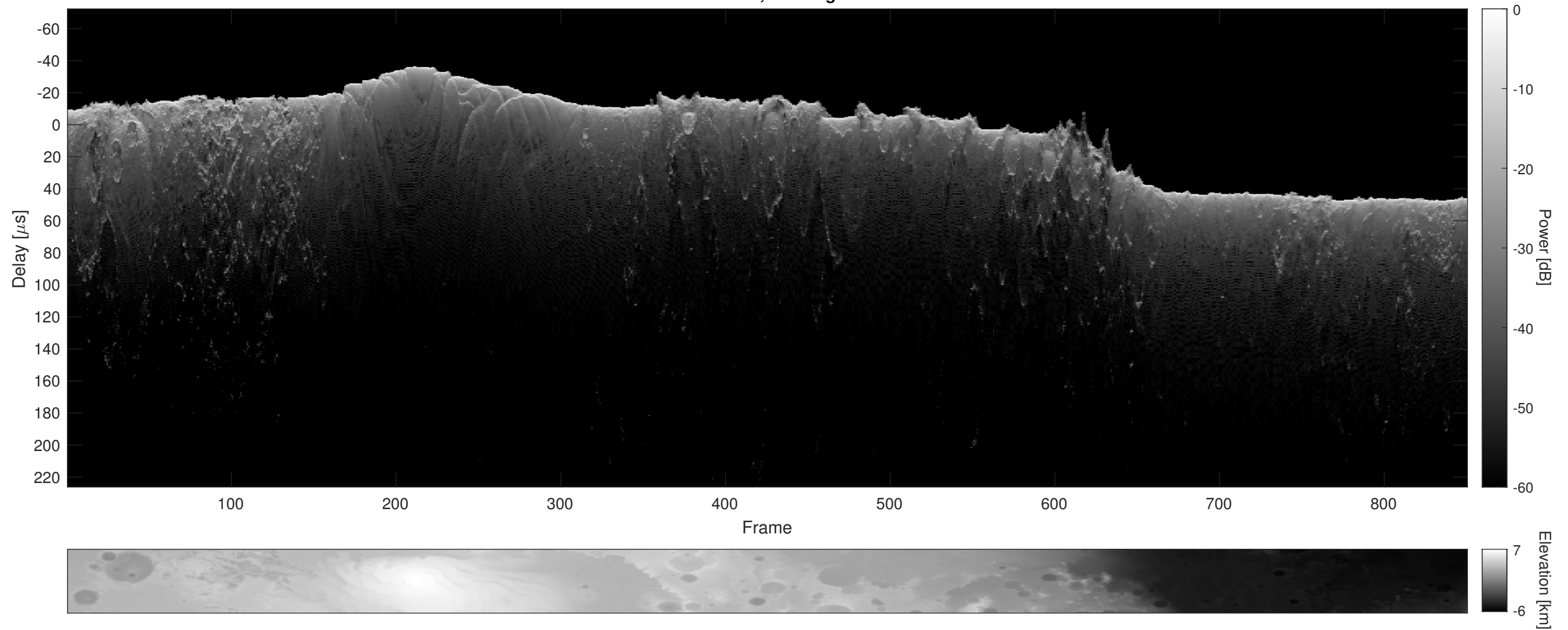
Orbit 14838, Cluttergram
