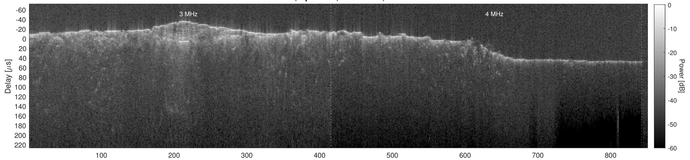
Orbit 14838, Cluttergram
