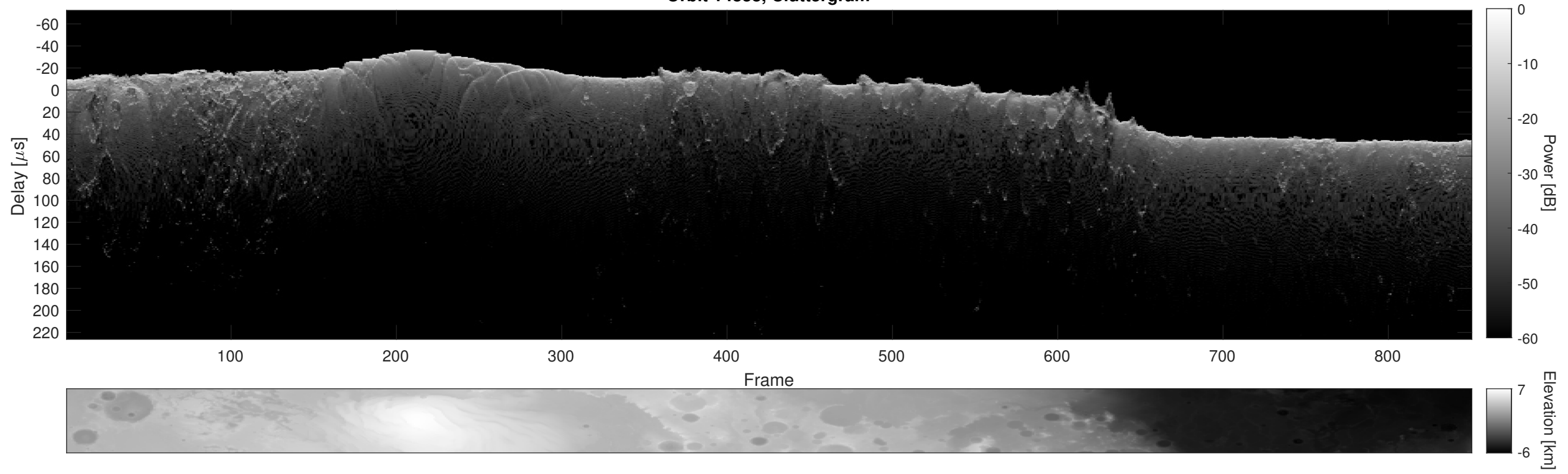
Orbit 14838, Cluttergram
