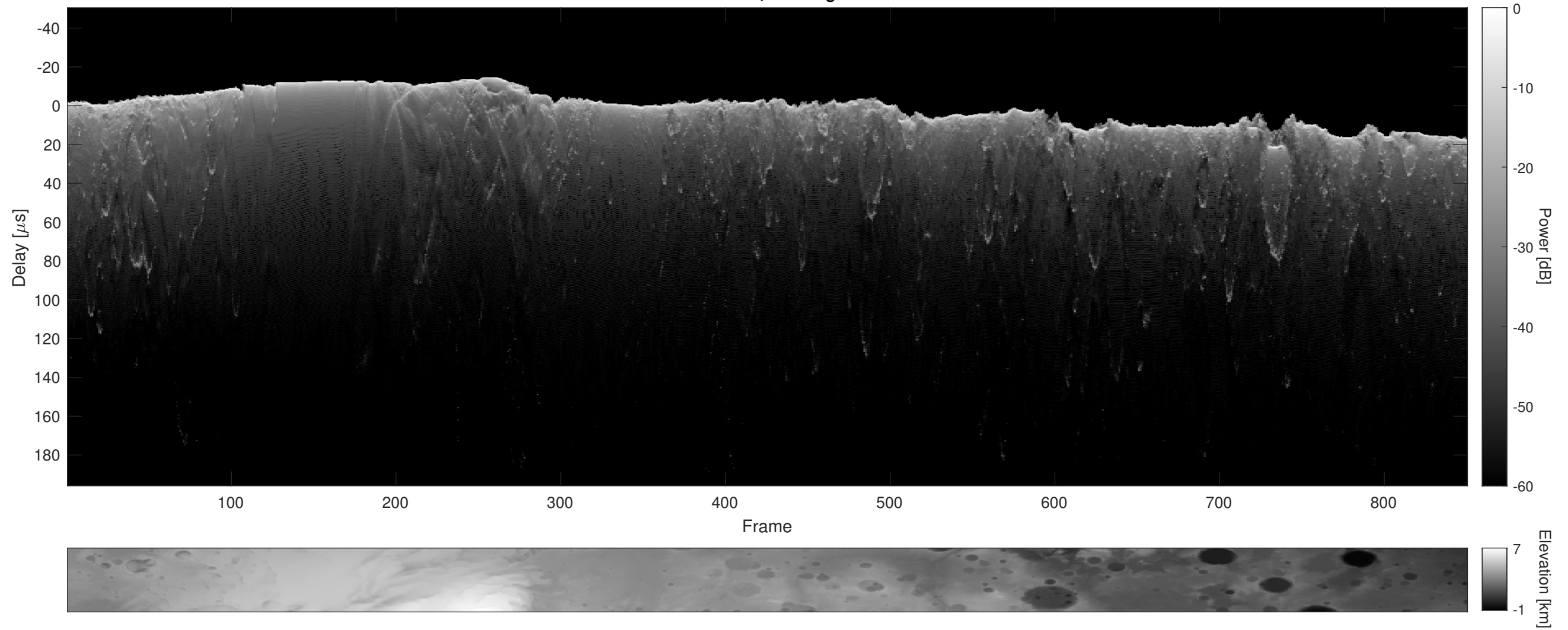
Orbit 14839, Cluttergram
