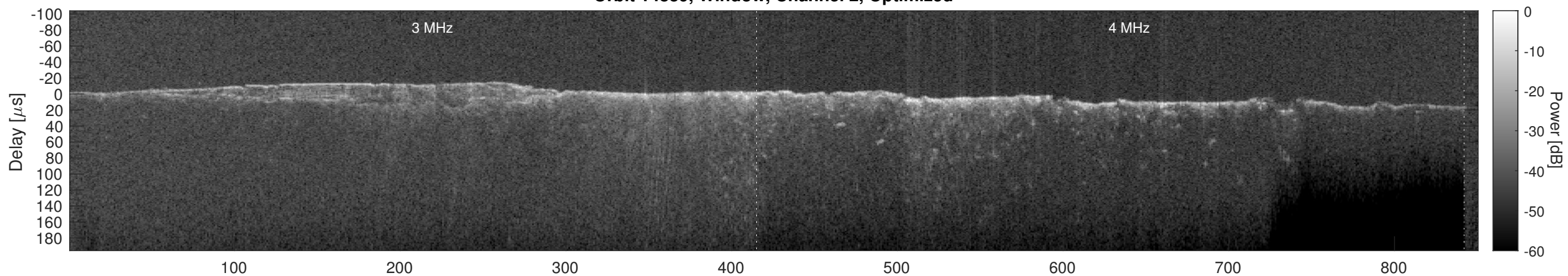
Orbit 14839, Cluttergram
