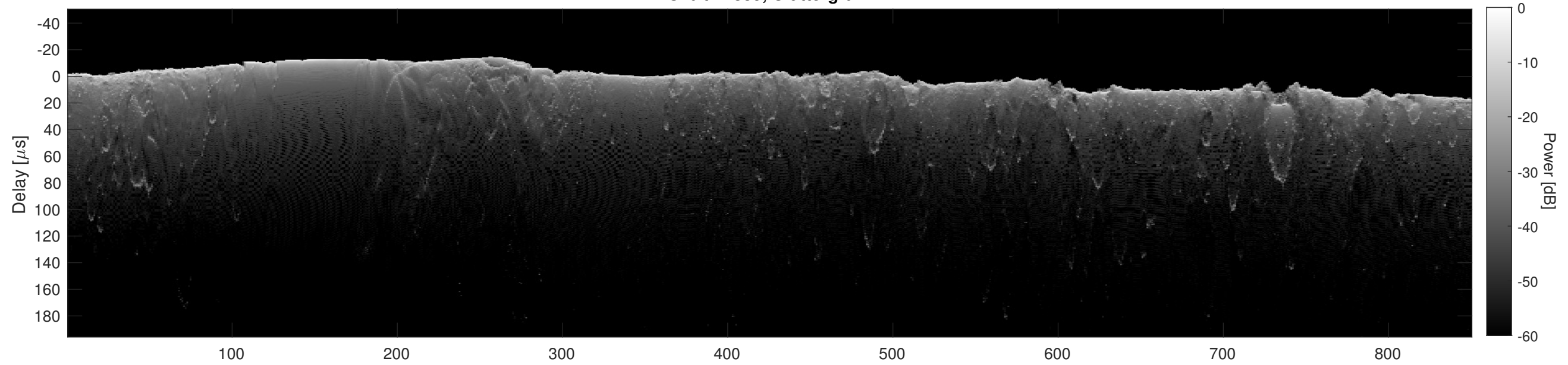
Orbit 14839, Cluttergram
