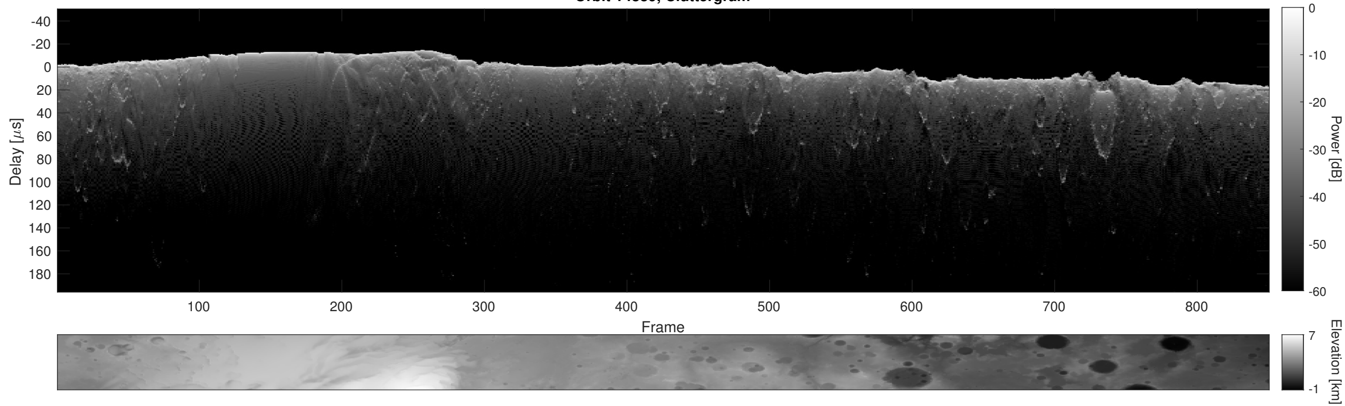
Orbit 14839, Cluttergram
