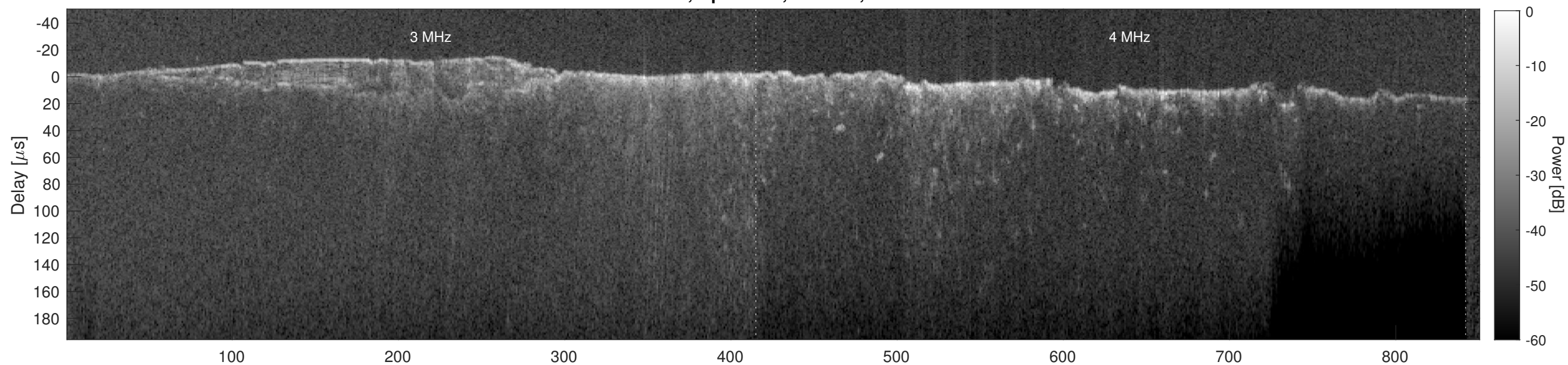
Orbit 14839, Cluttergram
