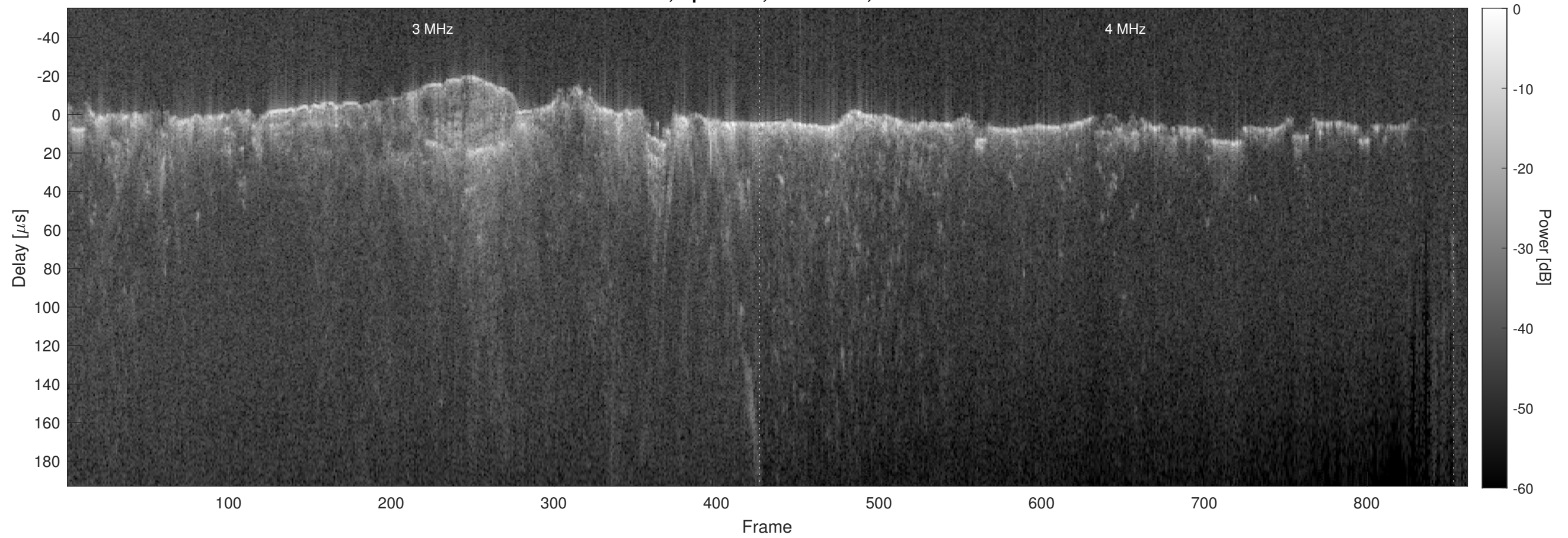
Orbit 14842, Optimized, No Window, Channel 2
