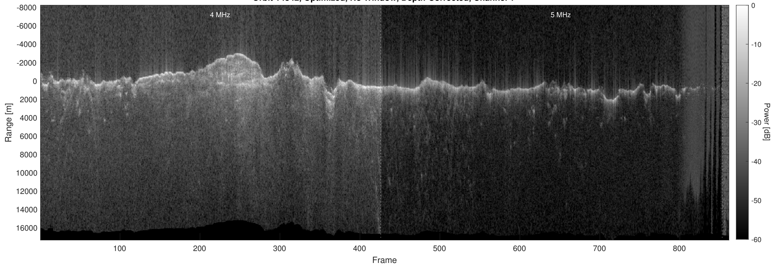
Orbit 14842, Optimized, No Window, Depth-Corrected, Channel 2
