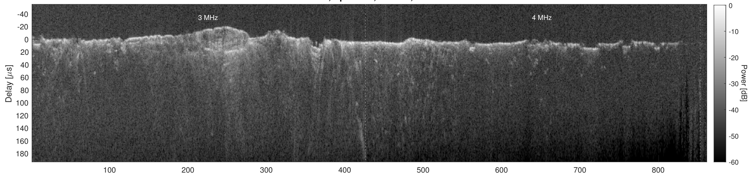
Orbit 14842, Cluttergram
