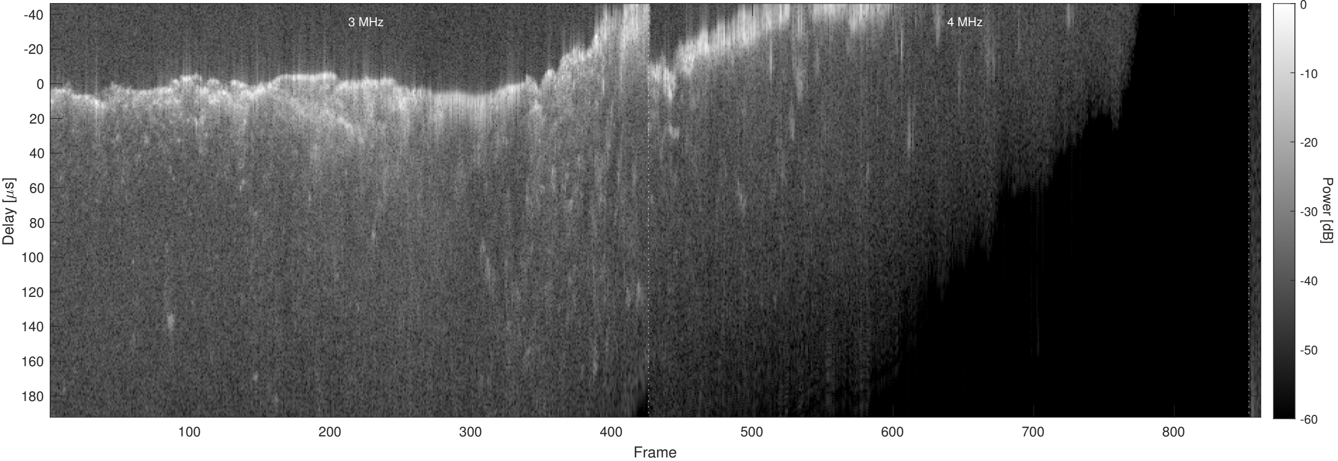
Orbit 14843, Chapman, No Window, Channel 2
