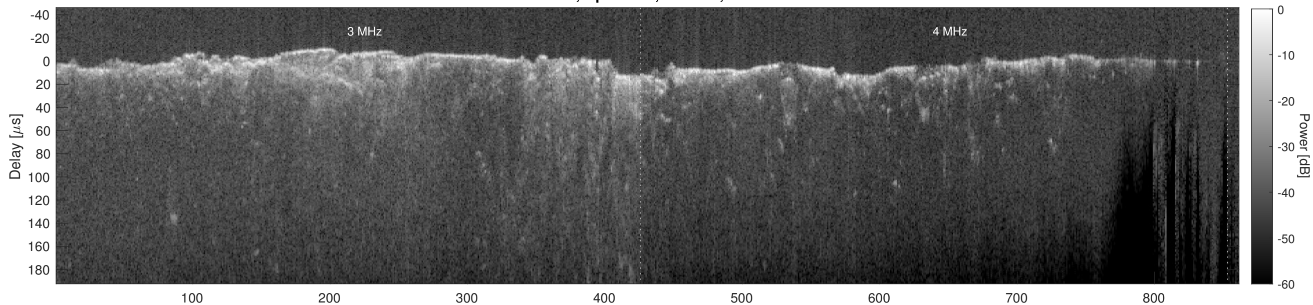
Orbit 14843, Cluttergram
