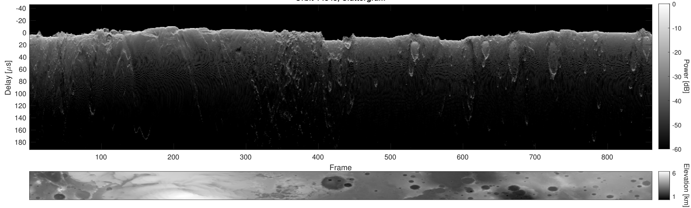
Orbit 14843, Cluttergram
