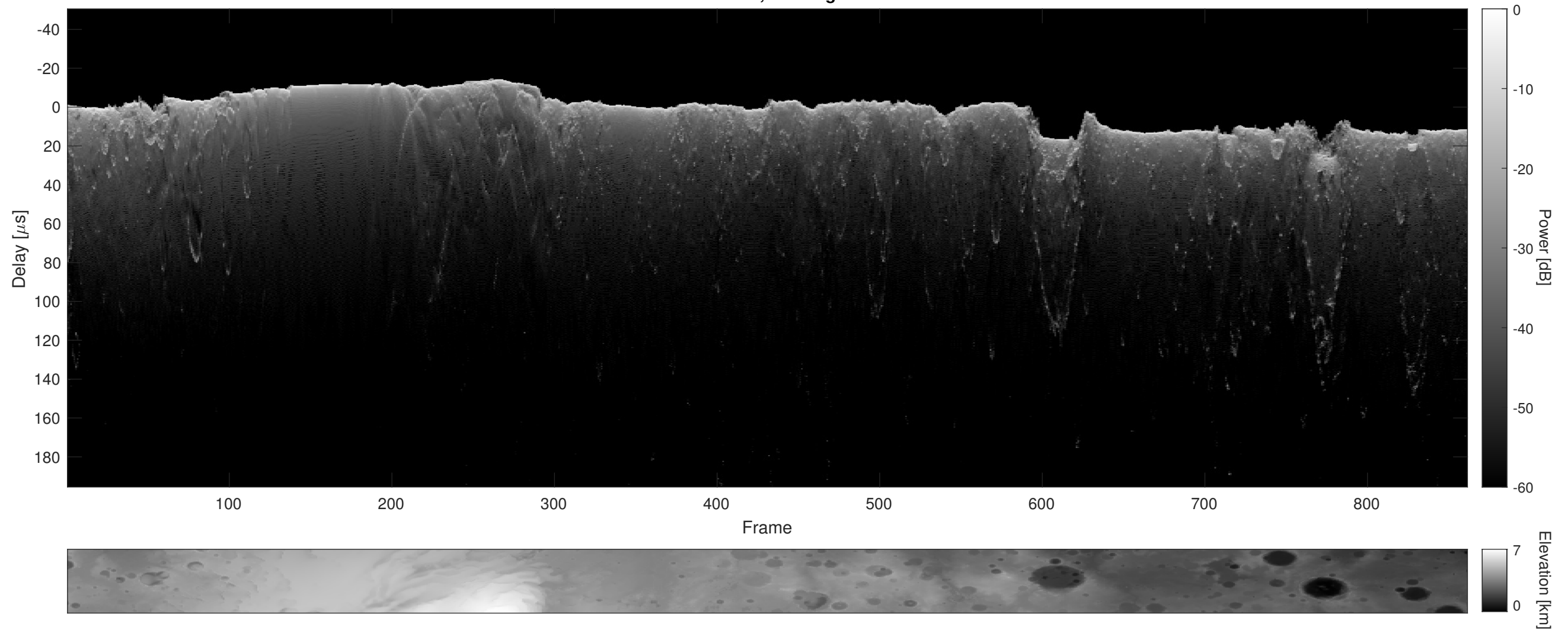
Orbit 14846, Cluttergram
