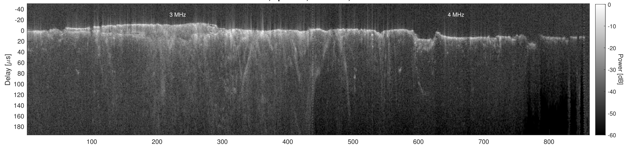
Orbit 14846, Cluttergram
