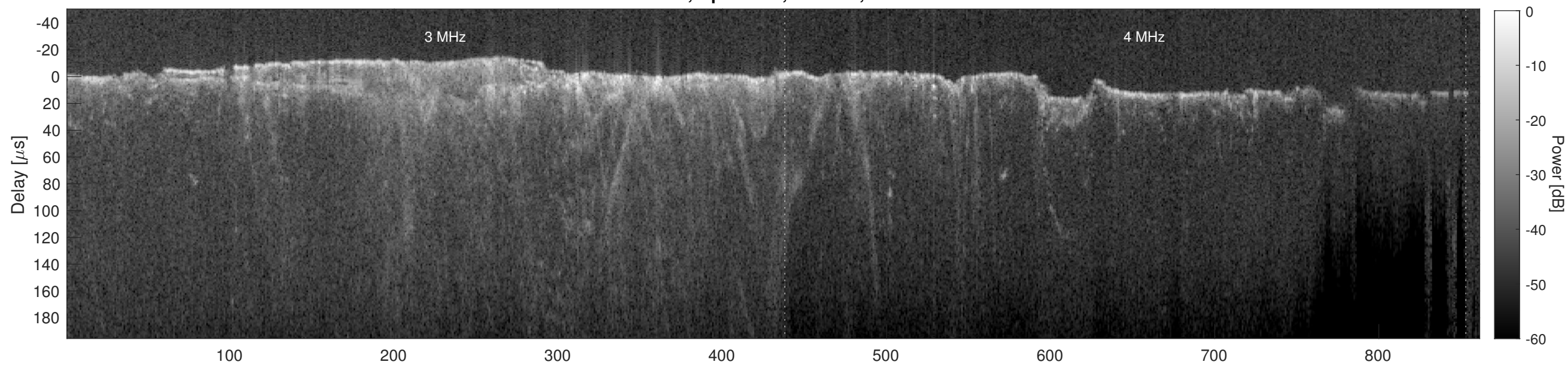
Orbit 14846, Cluttergram
