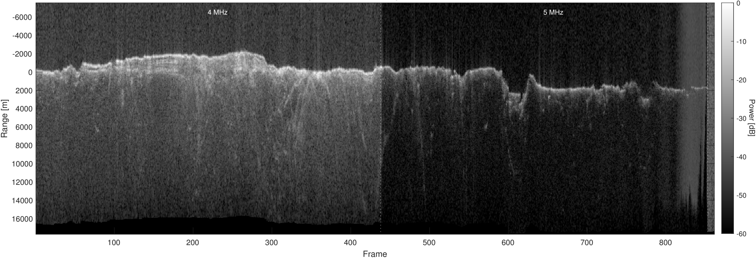
Orbit 14846, Optimized, Window, Depth-Corrected, Channel 2
