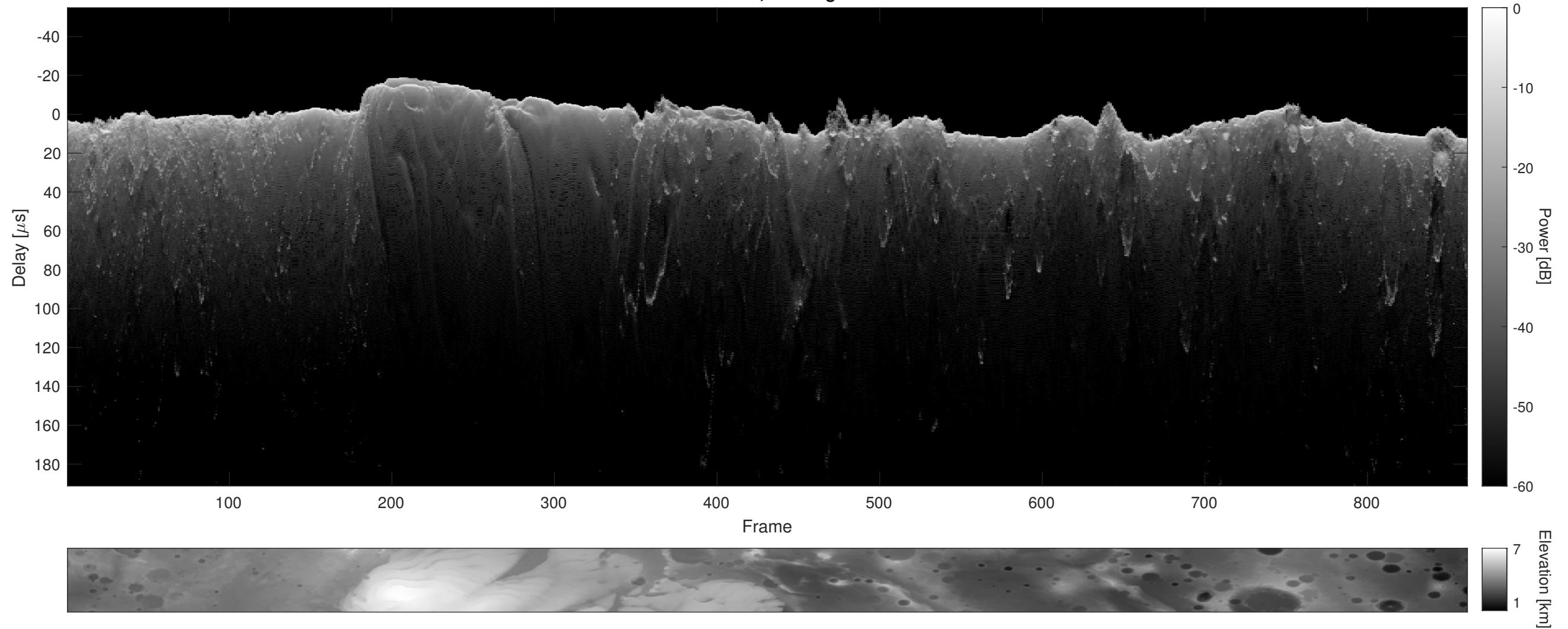
Orbit 14848, Cluttergram
