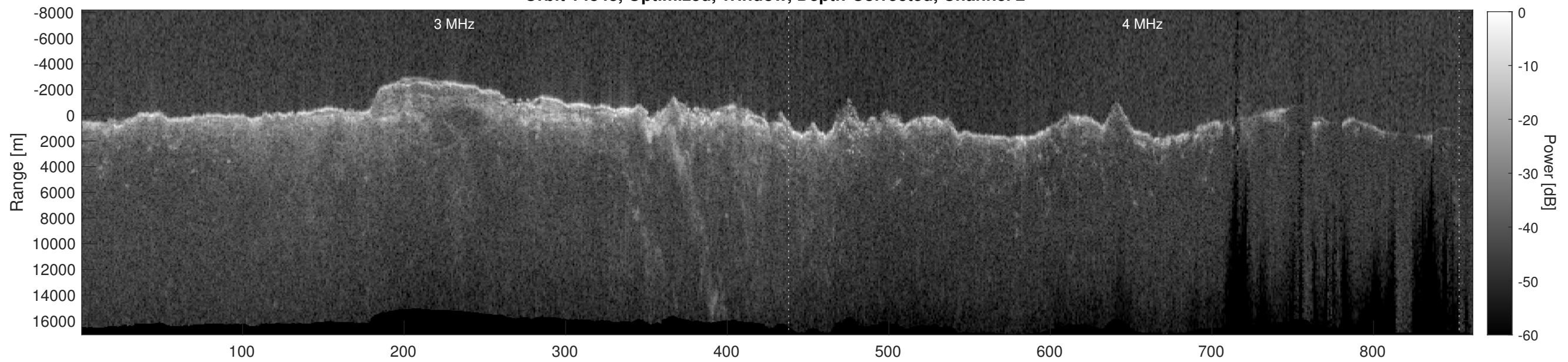
Orbit 14848, Depth-Corrected Cluttergram
