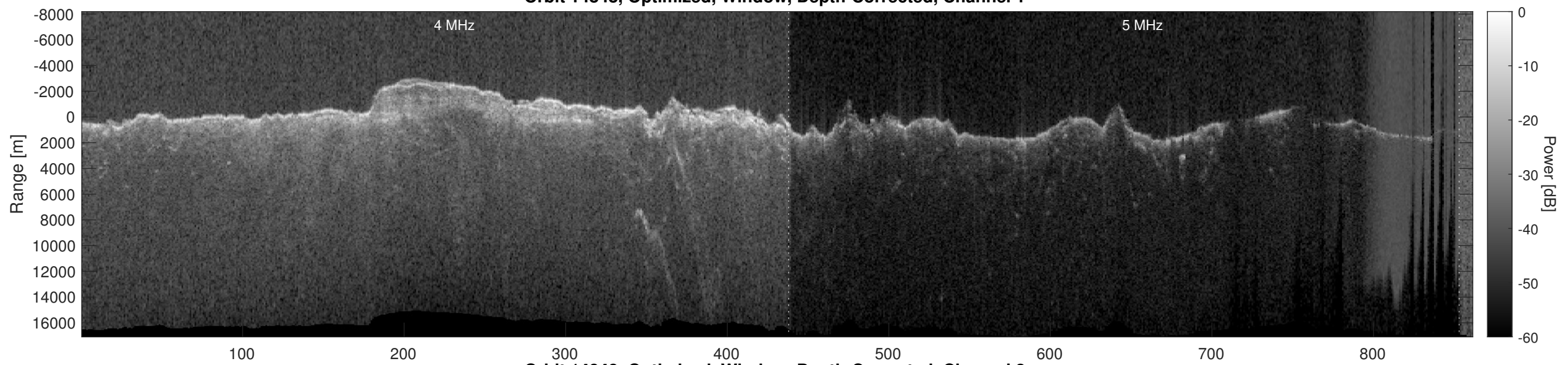
Orbit 14848, Optimized, Window, Depth-Corrected, Channel 2
