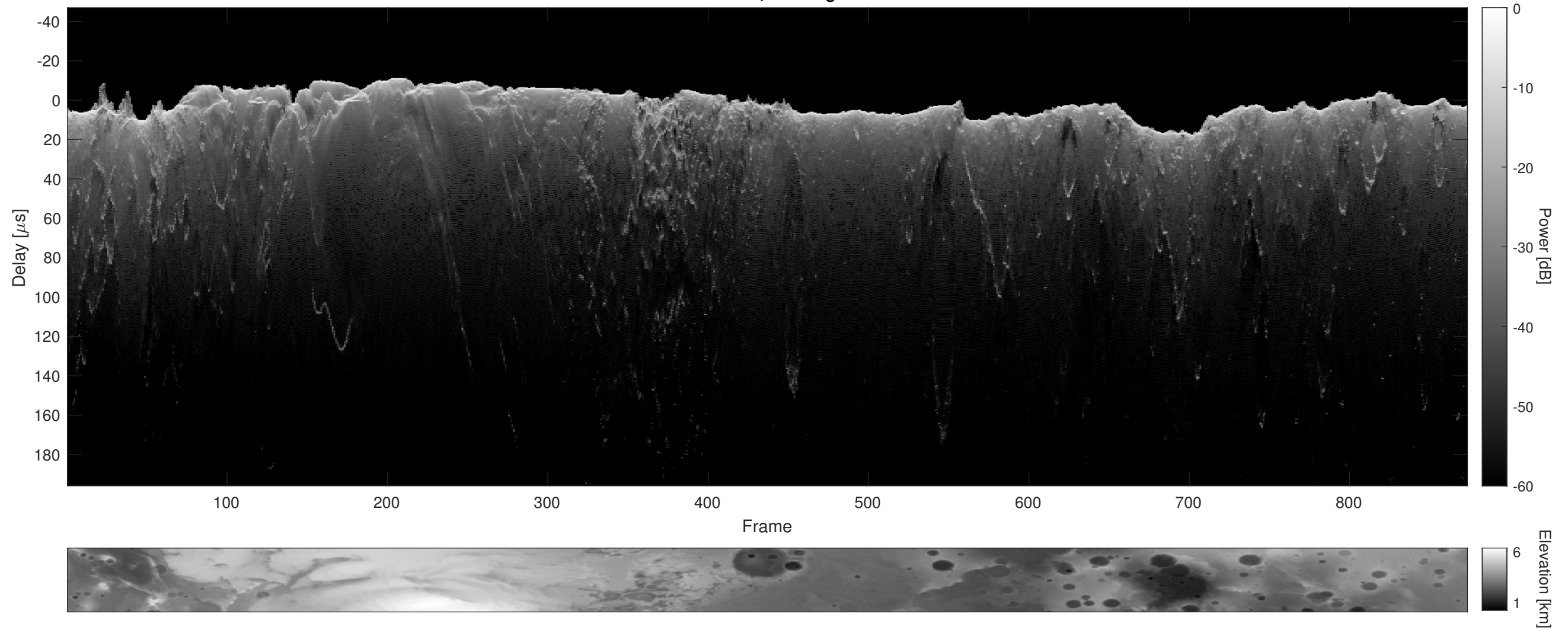
Orbit 14850, Cluttergram
