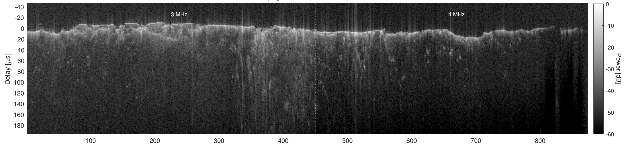
Orbit 14850, Cluttergram
