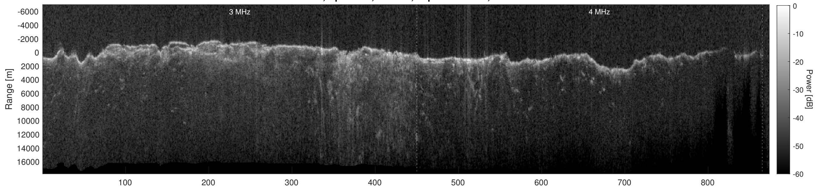
Orbit 14850, Depth-Corrected Cluttergram
