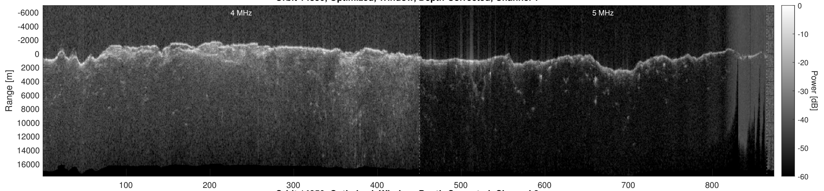
Orbit 14850, Optimized, Window, Depth-Corrected, Channel 2
