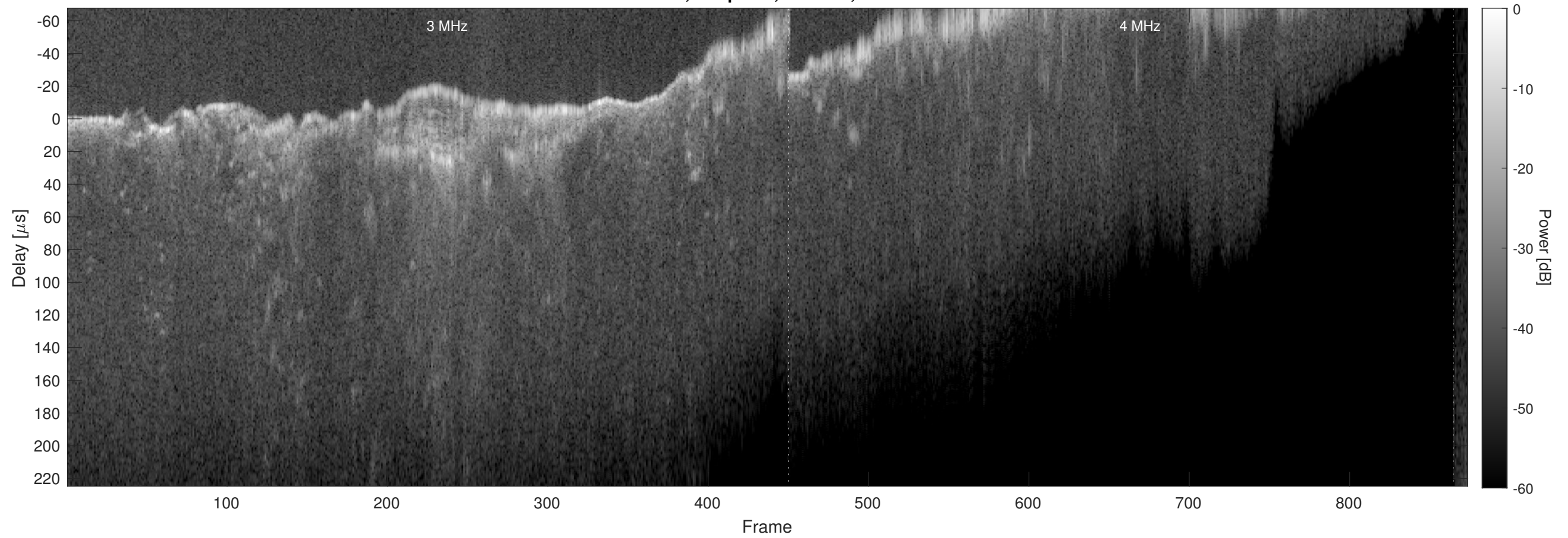
Orbit 14852, Chapman, Window, Channel 2
